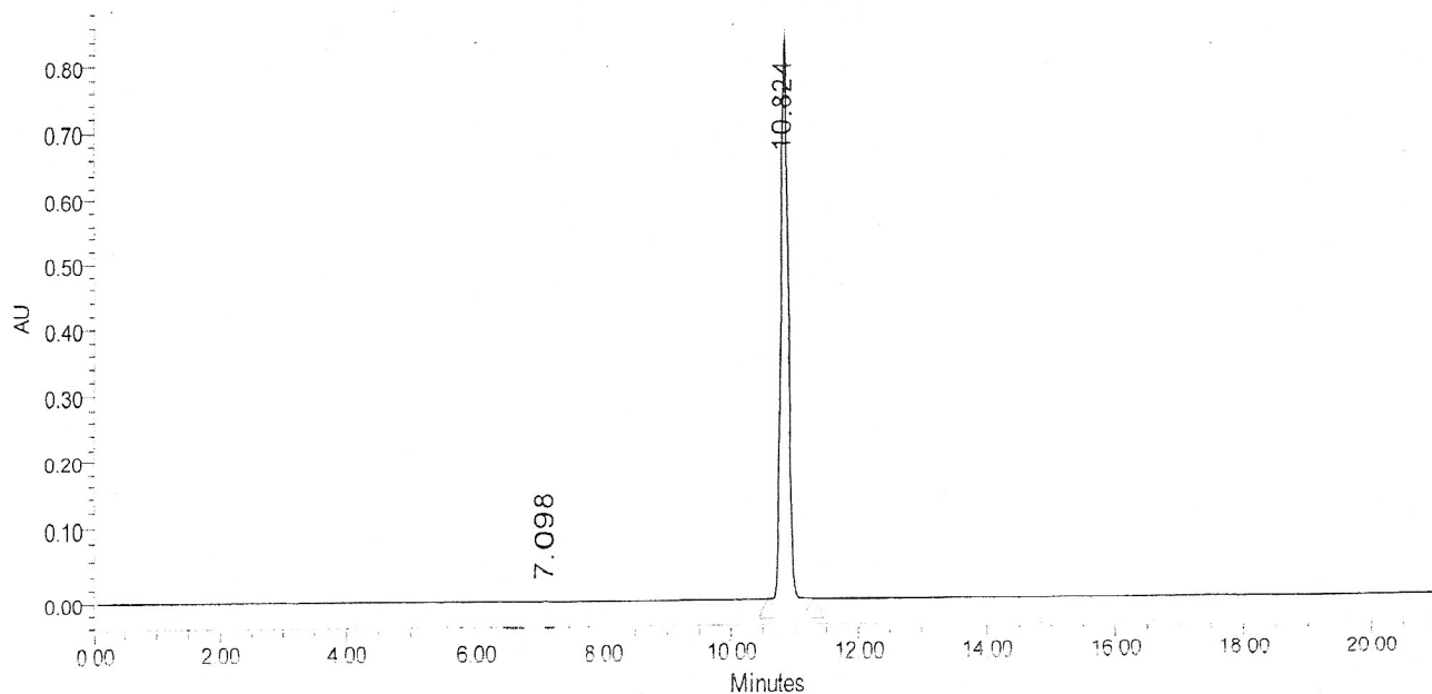
Auto-Scaled Chromatogram
